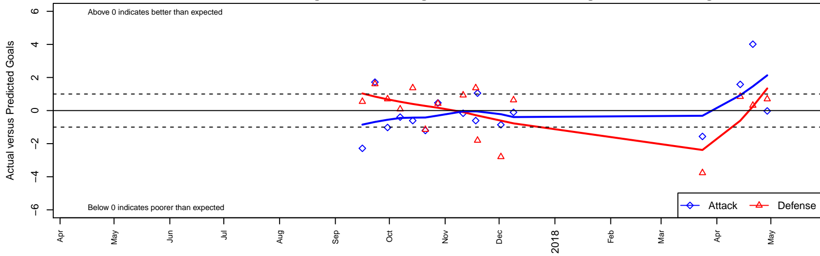
STU Evolution Trujillo B04 Dots are actual minus expected GF (blue circles) and GA (red triangles). Blue line is smoothed change in attack strength. Red is smoothed change in defense strength.
